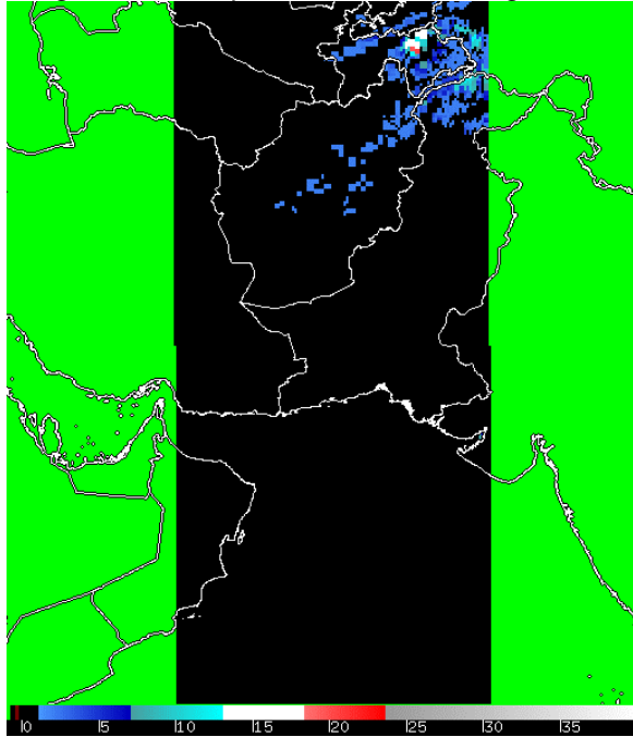
Figure 2. Oct 15, 2002, 06 GMT: DMSM SSM/I Snow Depth Estimate (inches).
